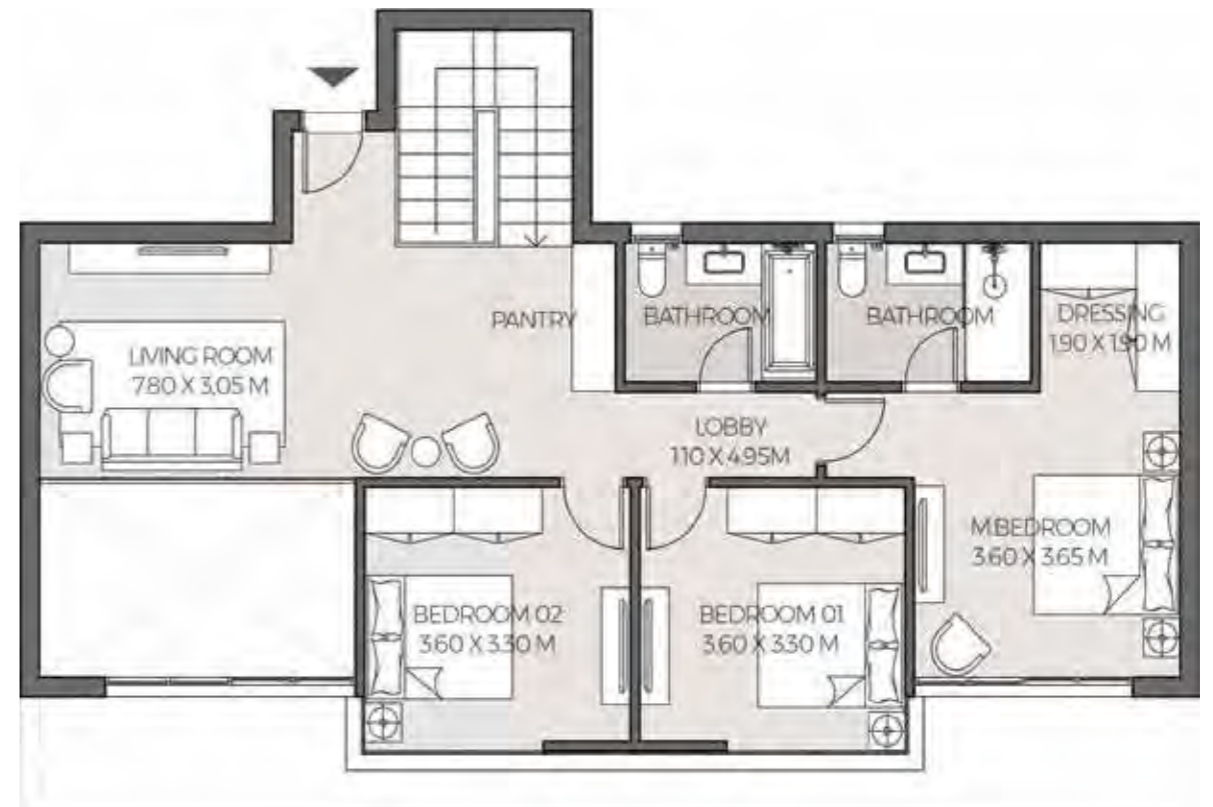
UPPER LEVEL
