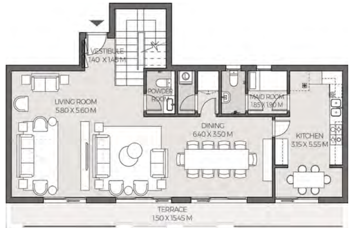
LOWER LEVEL
