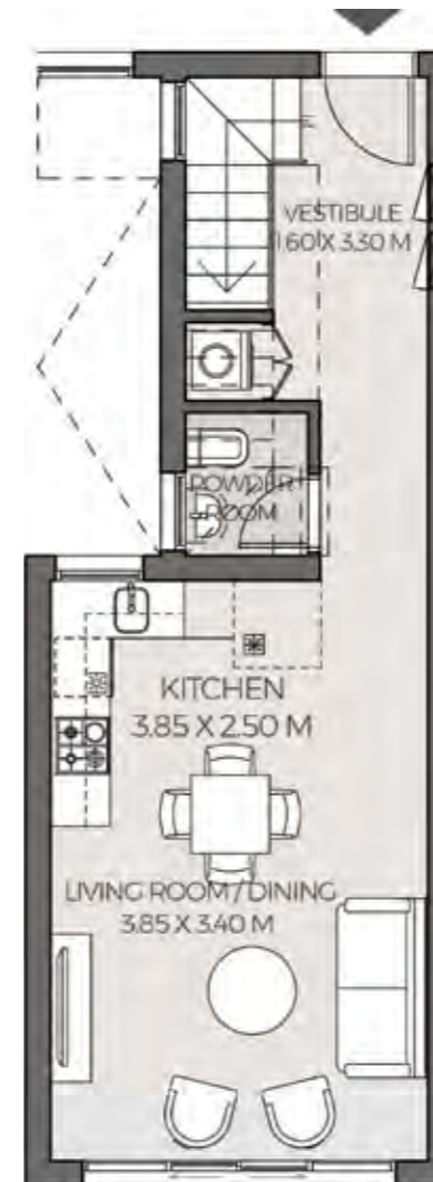
GARDEN LEVEL
